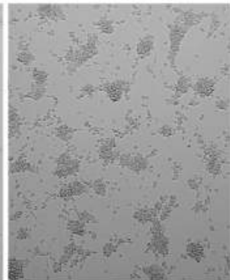
C ZIKV (MR766)
