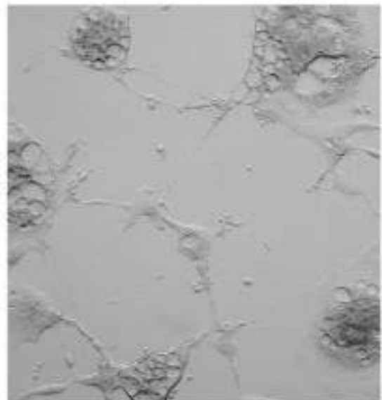
A DENV-1 (TH-Sman)
