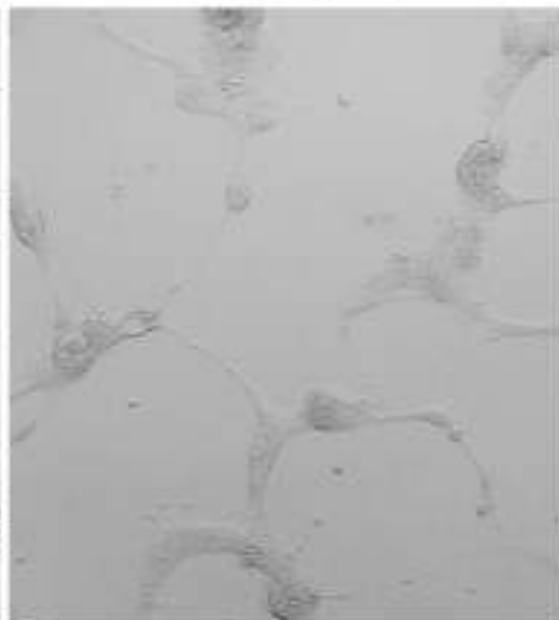
B DENV-2 (NGC)
