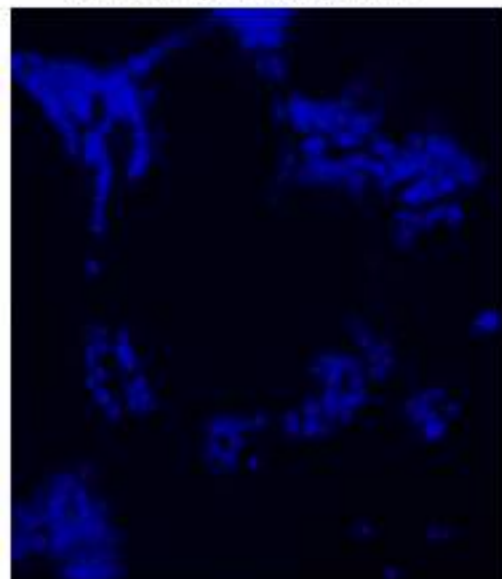
D DENV-1 (TH-Sman) DAPI
